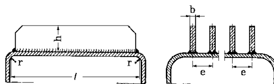
Figure 15.26 Arrangement of self-supported girders
