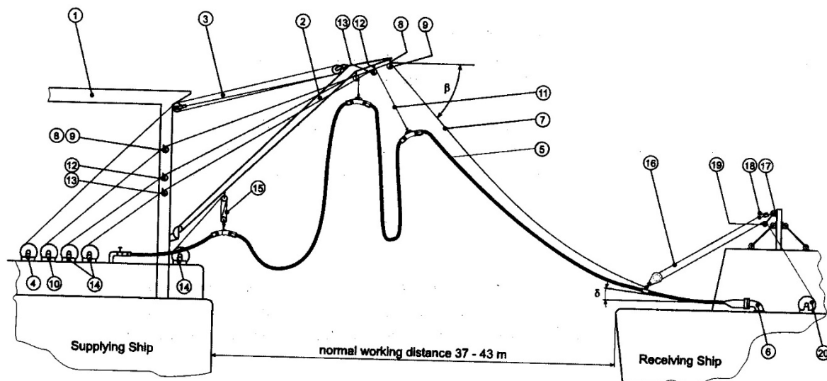
Figure 4.5 Large derrick system for liquid transfer
