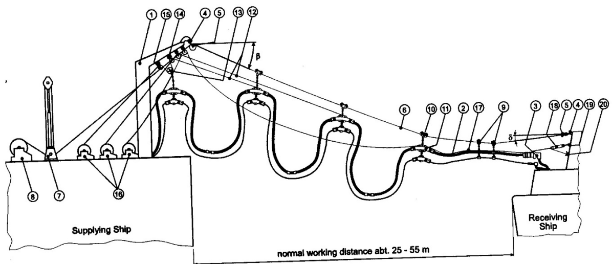
Figure 4.4 STREAM system for liquid transfer
