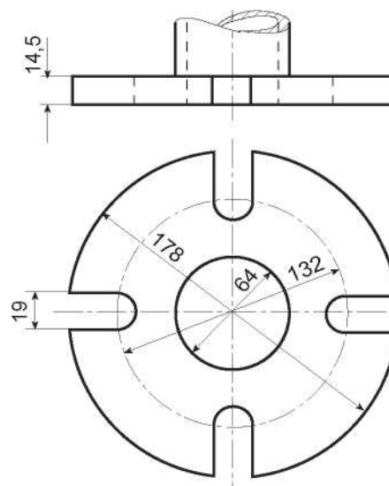
Fig. 9.1 International shore connection
