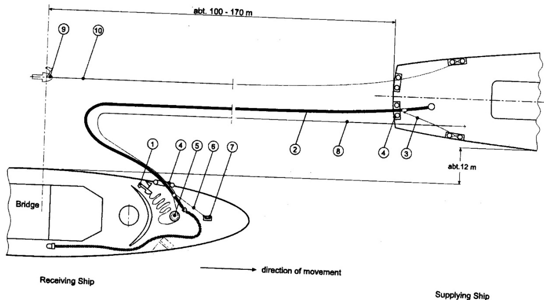
Figure 4.7 Stern /bow system for liquid transfer
