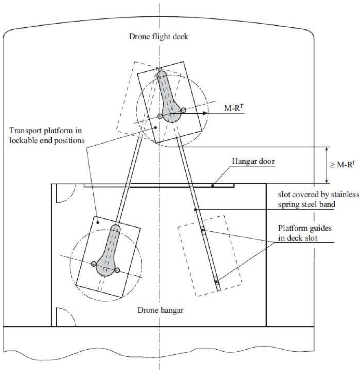
Figure 13.1 Example with the main characteristics of a safe drone handling
