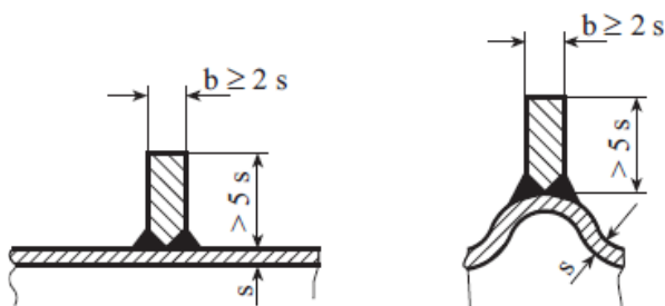
Fig. 15.4 Types of structure for stiffening
