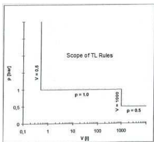
Fig. 16.1 Scope of BCS Rules for pressure vessels
