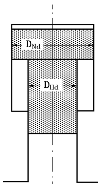
Figure 6.3 Cylinder bores for compressors with a differential piston
