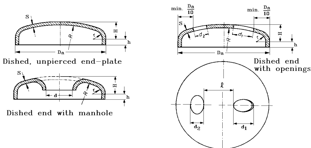
Fig. 15.6 Parameters for unstayed dished end plates
