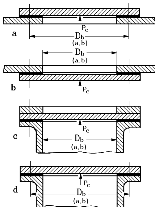
Figure 15.12 Circular plates with flat sealing
