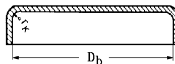
Figure 15.11 Flat, circular flanged endplates
