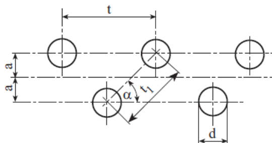
Figure 15.25 Arrangement of staggered rows of holes
