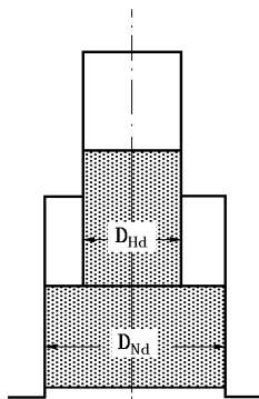
Figure 6.2 Cylinder bores for compressors with a stepped piston
