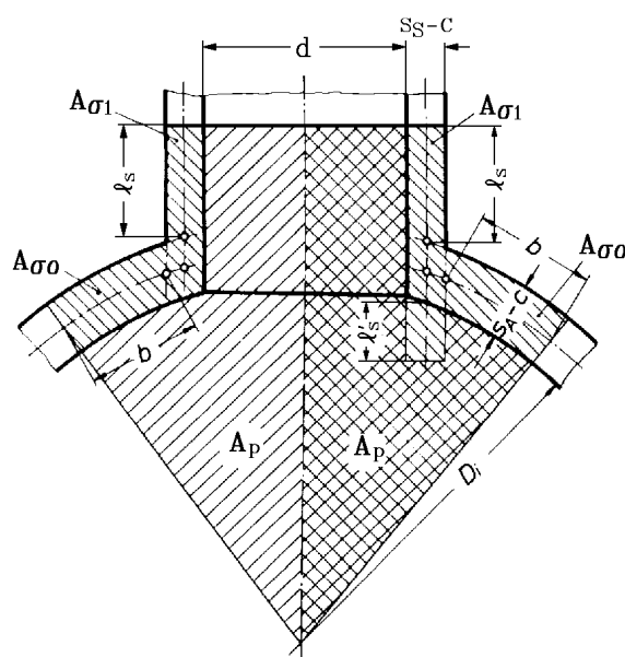
Fig. 15.8 Openings in dished end plates (Areas A_p and A_\sigma )
