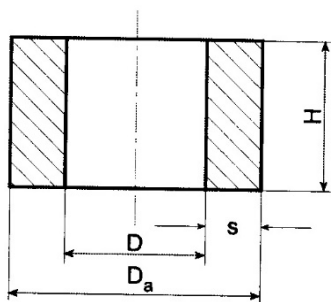
Fig. 2.1 Hub dimensions
