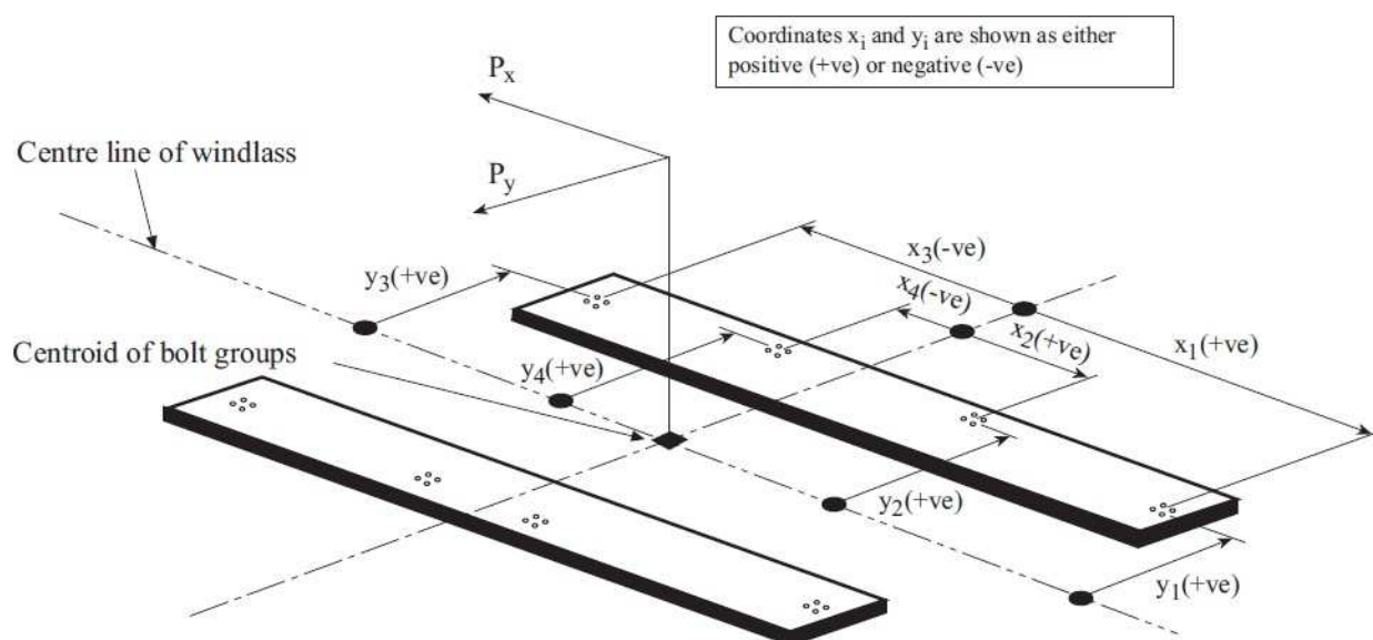
Figure 5.2 Sign convention
