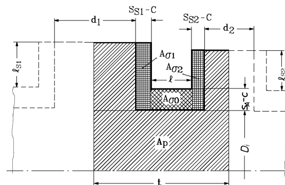
Fig. 15.3 Mutual effect on openings
