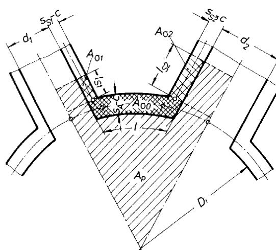
Fig. 15.9 Mutual effect of openings
