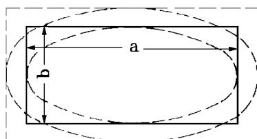
Figure 15.15 Parameters of rectangular and elliptical plates
