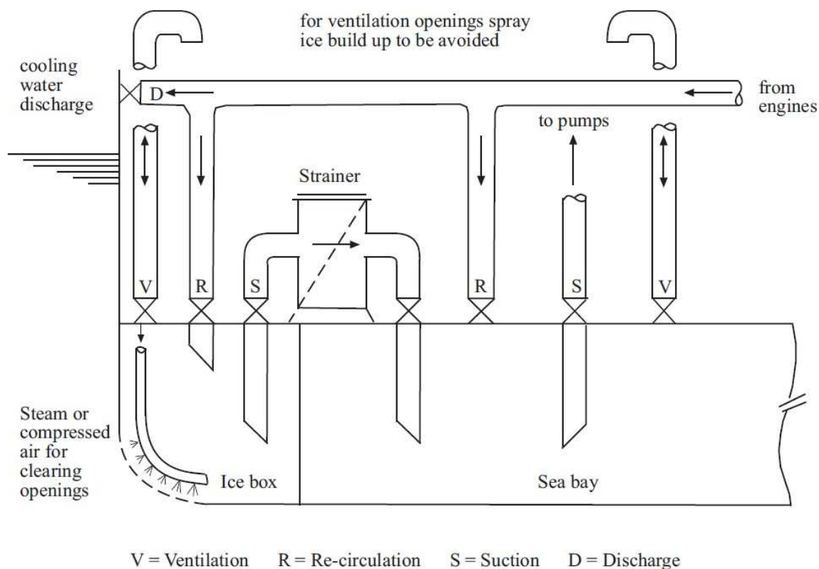
Figure 19.1 Suggested arrangement of seawater inlet system (IMO suggested arrangement)
