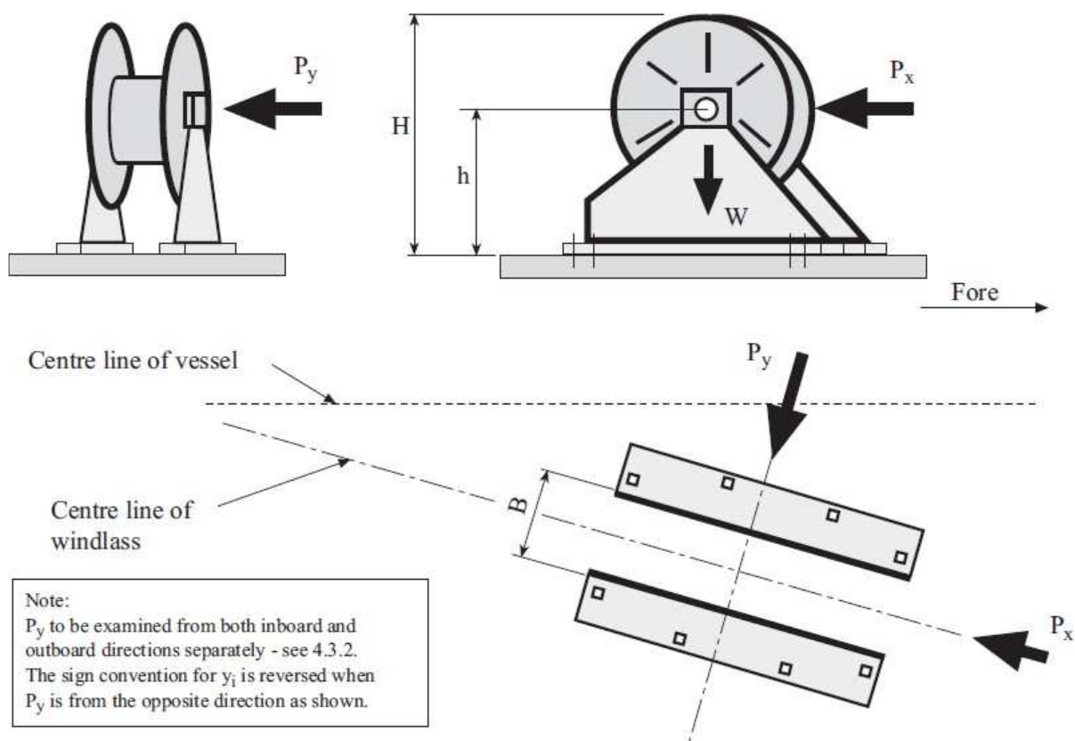
Figure 5.1 Direction of forces and weight
