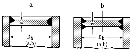
Figure 15.14 Circular welded-in endplates
