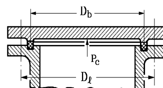
Figure 15.13 Circular plate with sealing ring
