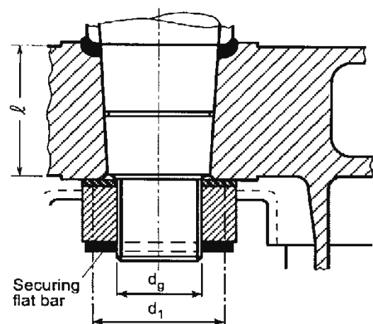
Figure 12.10 Cone coupling with special arrangements for mounting and dismounting
