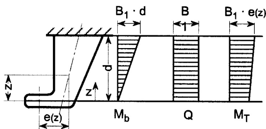
Figure 12.6 Forces on the rudder horn
