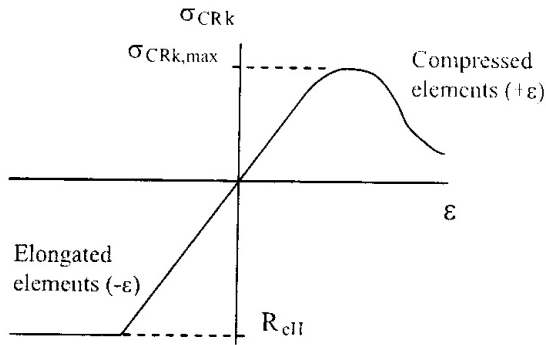
Figure 6.8 Typical average stress-average strain curve
