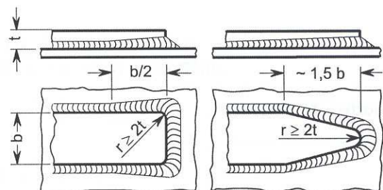
Figure 15.4 Welding at the ends of doubling plates
