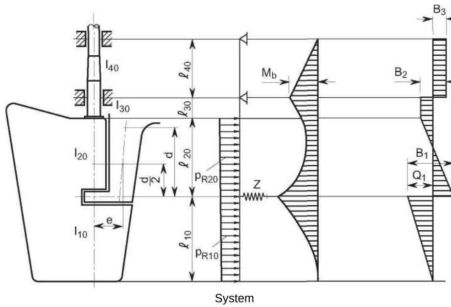
Figure 12.3 Semi-spade rudder
