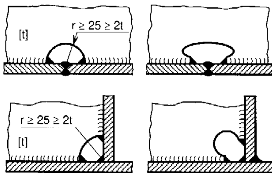
Figure 15.3 Welding cut-outs
