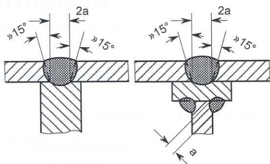
Figure 15.13 Three plate connection
