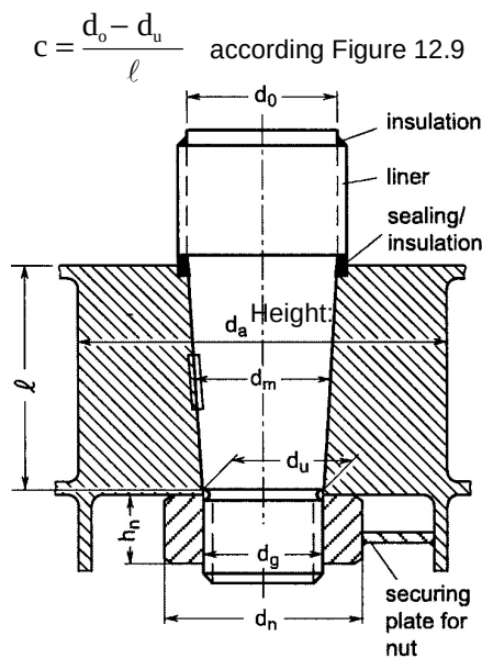
Figure 12.9 Cone coupling
