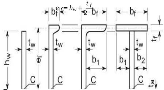
Figure 4.8 Main parameters of typical sections
