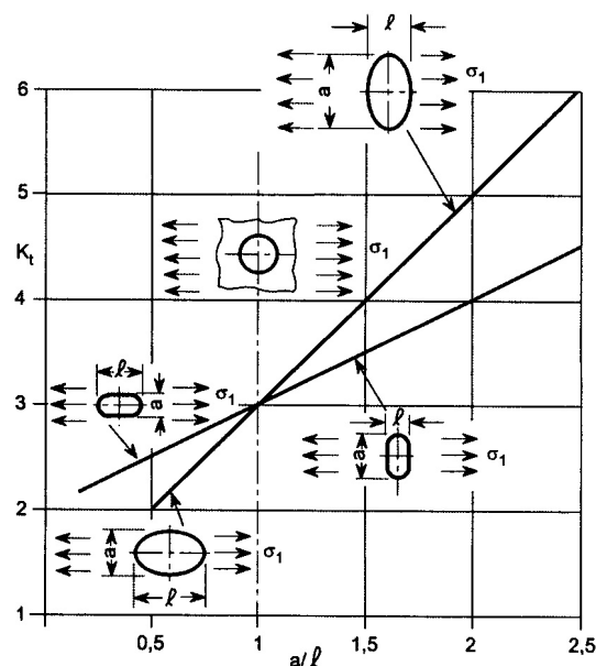
Figure 4.11 Notch factor K_t for rounded openings
