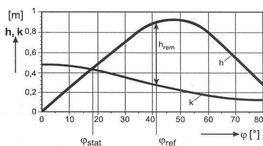
Fig. 2.1 Lever arm curves
