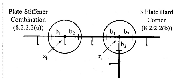
Figure 6.9 Structural elements
