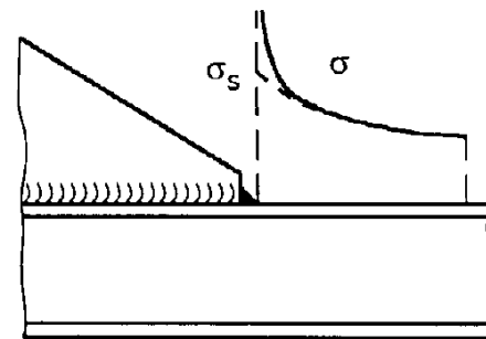
Figure 17.5 Structural stress
