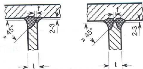
Figure 15.9 Single and double-bevel welds with defined incomplete root penetration
