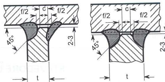
Fig. 15.10 Single and double-bevel welds with unwelded root face and defined incomplete root penetration
