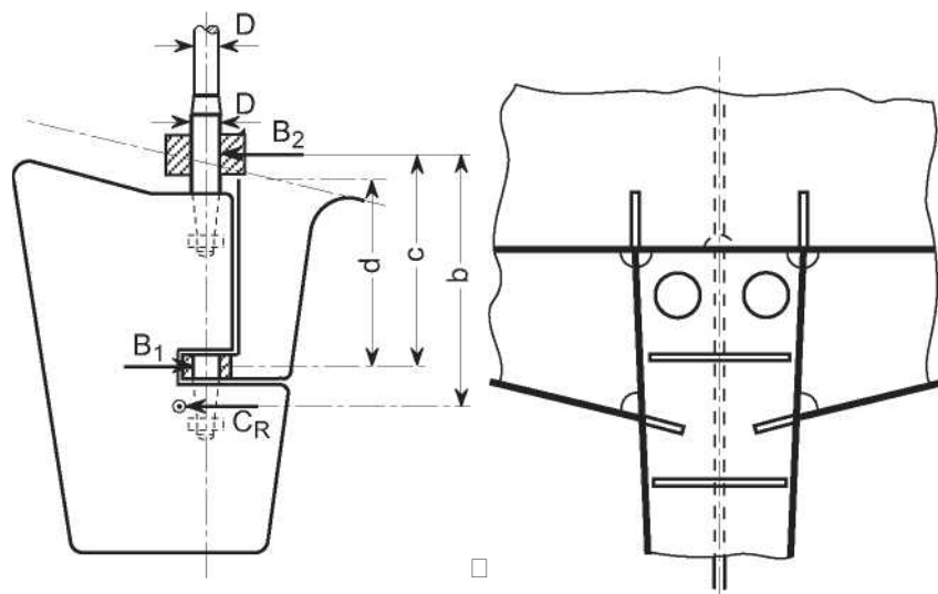
Figure 12.5 Parameters for semi spade-rudders
