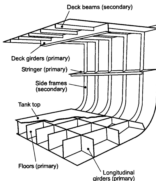
Figure 4.2 Definitions of primary and secondary stiffening members of the hull structure (transverse framing system)
