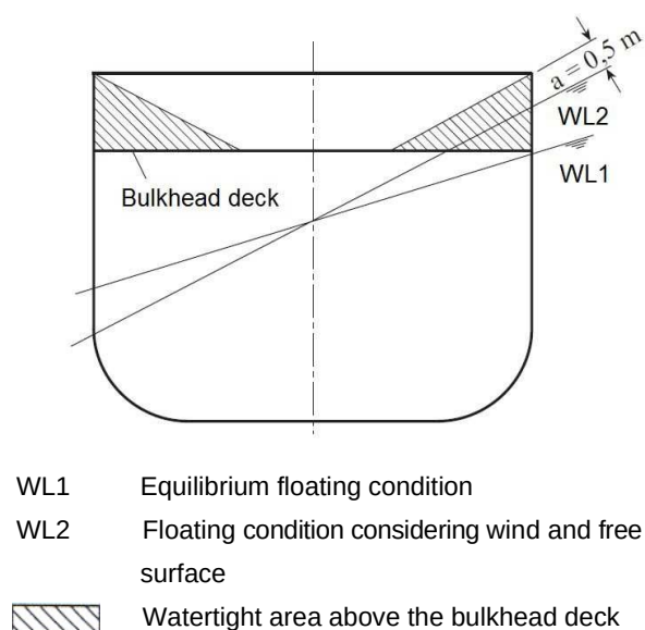
Fig. 2.2 Cross section at a watertight bulkhead
