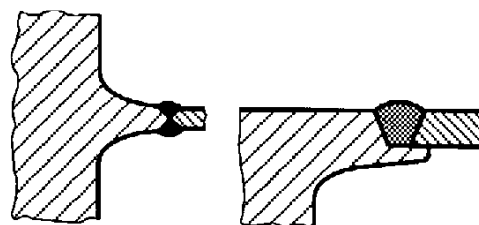
Figure 15.2 Welding flanges on steel castings of forgings
