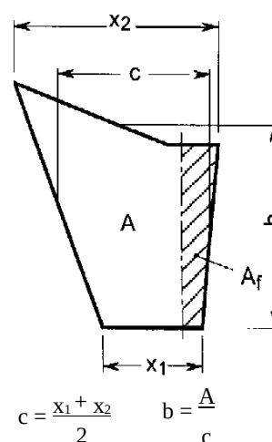
Figure 12.1 Rudder area
