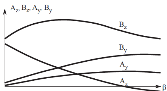
Figure 8.1 Support forces
