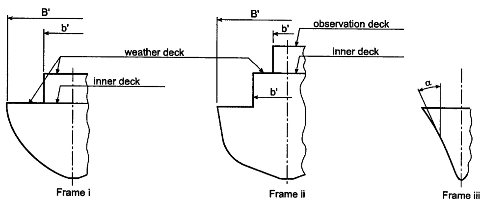
Figure 5.2 Definition of different parts of the ship's surface exposed to the sea
