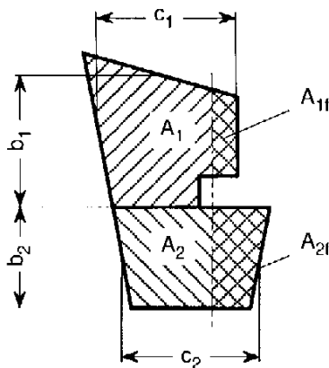
Figure 12.2 Rudder areas
