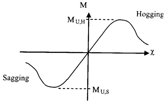
Figure 6.7 Moment-curvature curve
