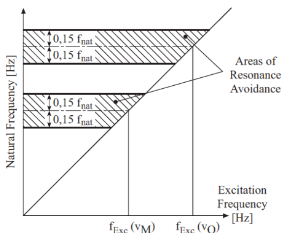
Figure 16.1 Resonance diagram
